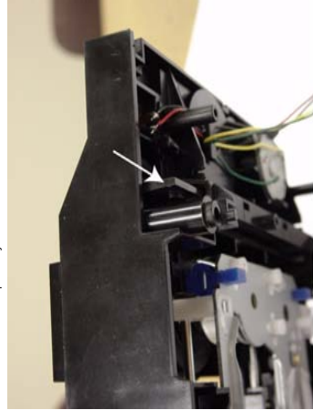
When a disc is loaded, unlock the tray by pushing the slide inwards by way of a screwdriver and pull tray outwards. Remove 4 screws to remove loader.
